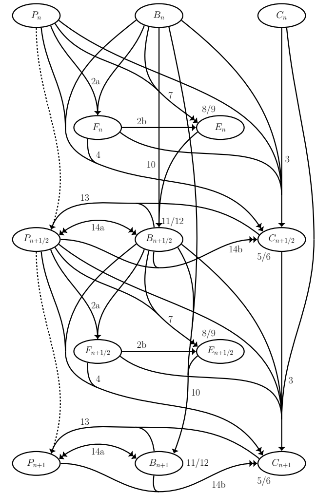
2nd-Order Runge-Kutta
